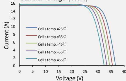
Current-Voltage (460W)
